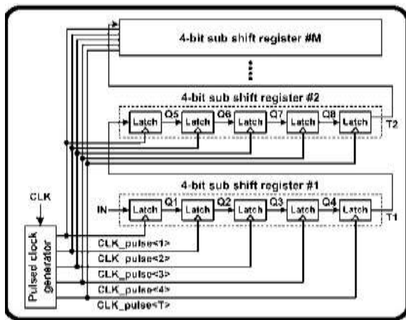
Fig.1. Block diagram of proposed shift register
